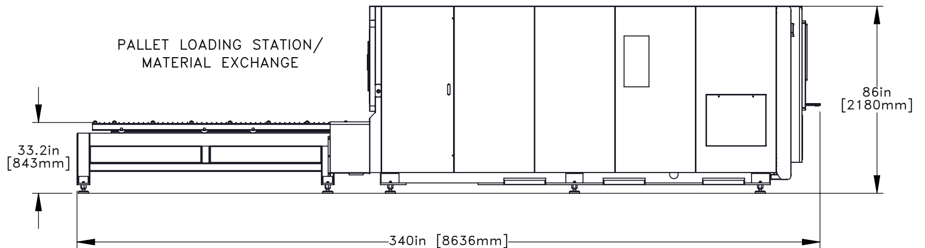
SIDE VIEW
