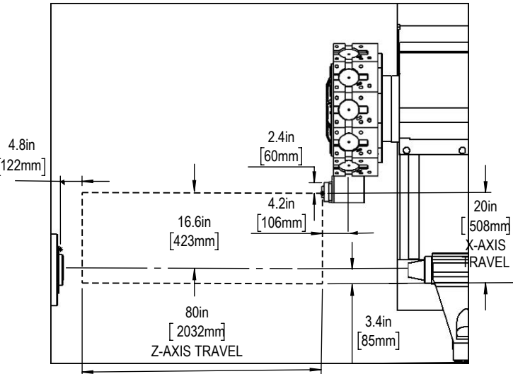
Optional Live Tooling - BMT75-90-DEGREE
