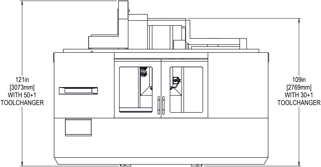
FRONT VIEW
