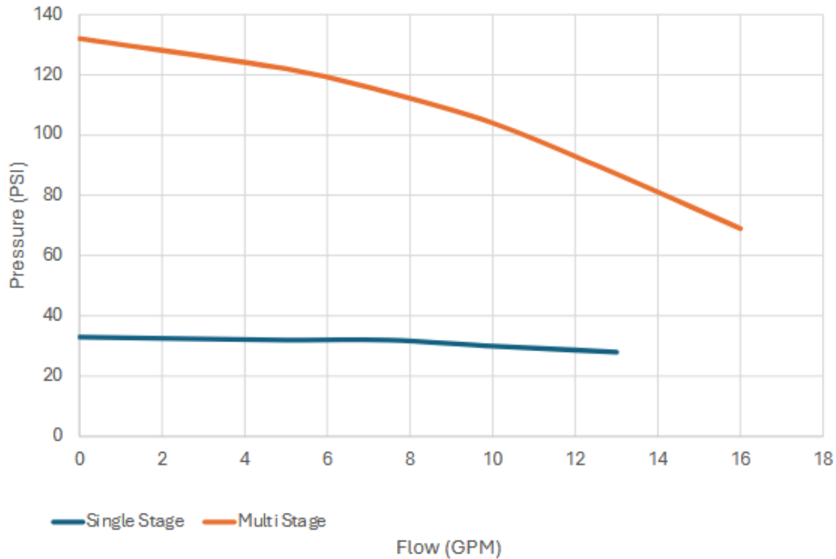
Multi vs. Single Stage Pump
